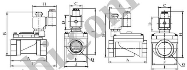
Dimensions (mm)
